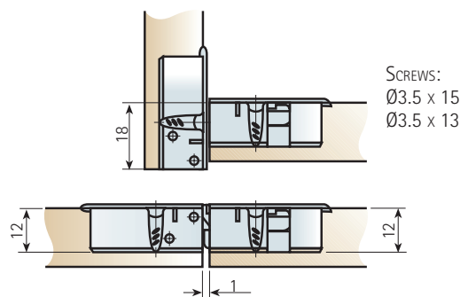
DEPTH ADJUSTMENT
