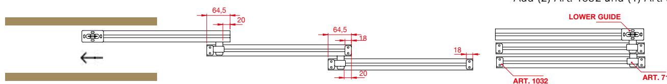
2-Leaf Sliding Door
